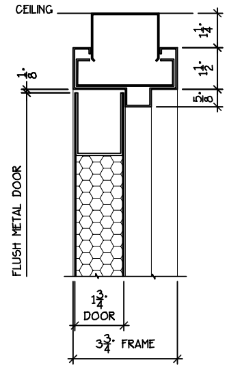
DOOR / FRAME HEADER AT CEILING
