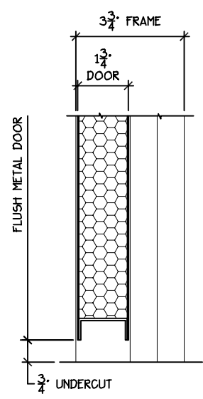
DOOR / FRAME UNDERCUT AT FLOOR
