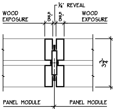
FLUSH WOOD PANEL AT INTERMEDIATE MULLION
