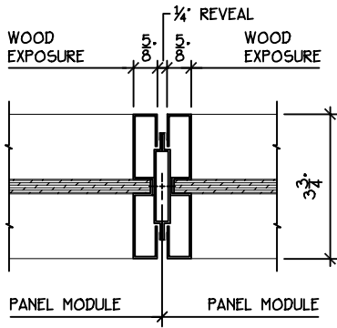
RECESSED WOOD PANEL AT INTERMEDIATE MULLION
